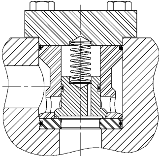
Check Valve Pocket Mount
