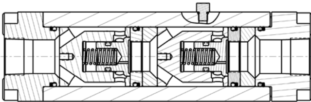
Double Check Valve - In-Line
