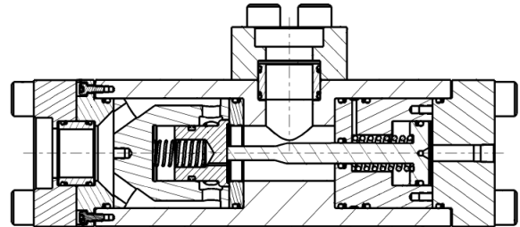
POCV, Socket Weld Ports
