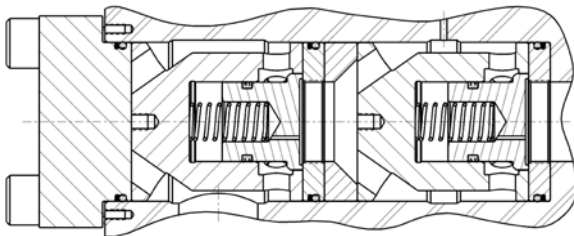
Double Check Valve - Pocket Mount
