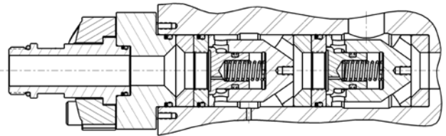
Double Check Valve - SAE Male - Pocket
