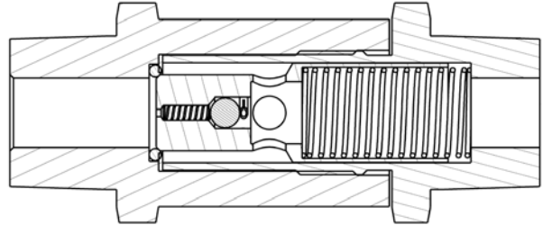
Check Valve w/Excess Flow/Bleed
