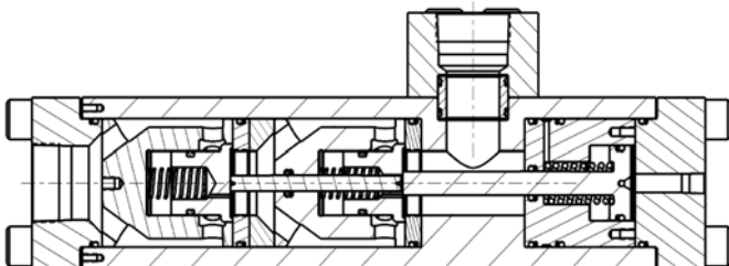
Double POCV, NPT Ports
